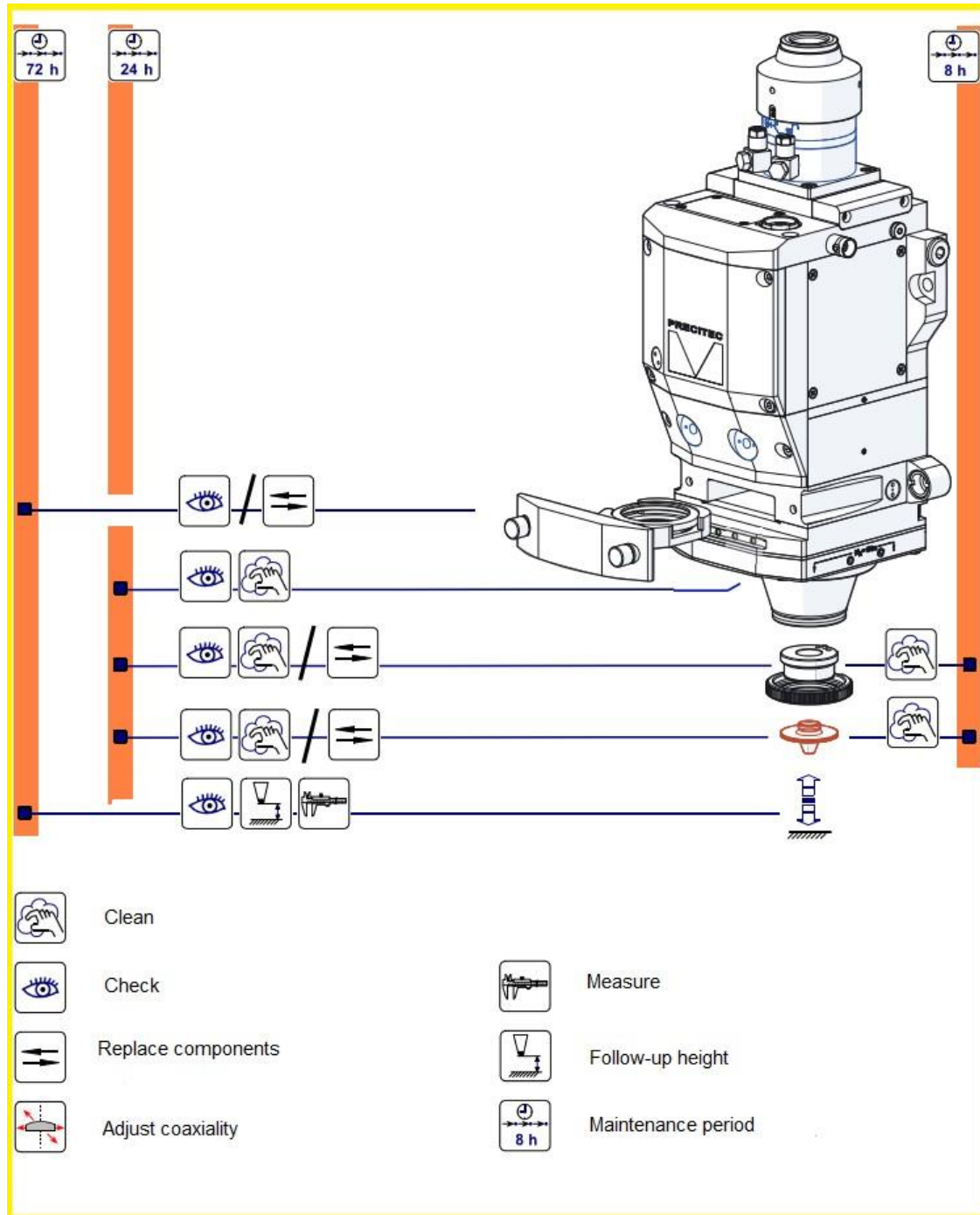
Maintenance Diagram for Cutting Head
